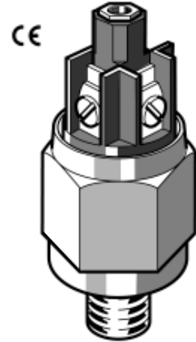
VCM1 with optional CAP 3 (IP65)
